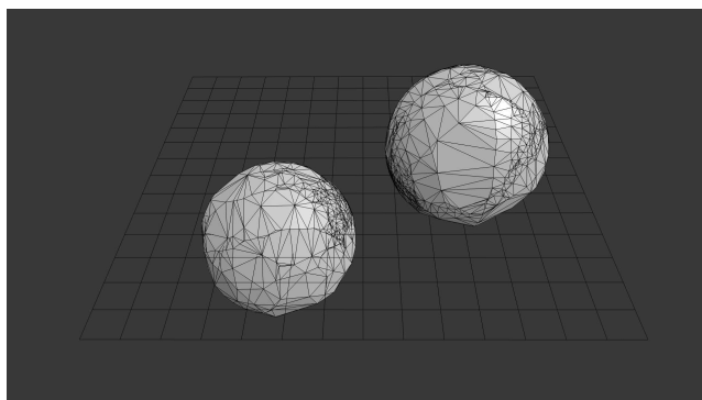
Fig. 3. Convex hull of the endpoints
