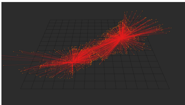
Fig. 1. Extended hedgehogs (Balázs Holl’s survey)
