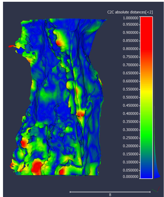
Fig. 10. Deviation of point cloud samples
