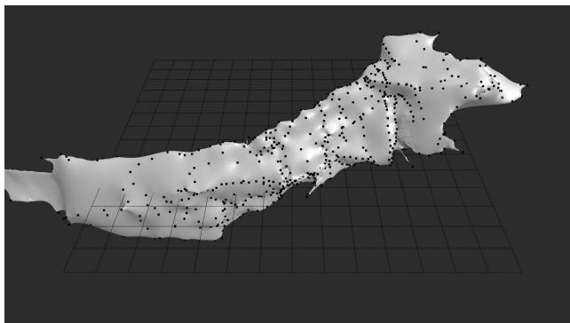
Fig. 6. Final biharmonic surface
