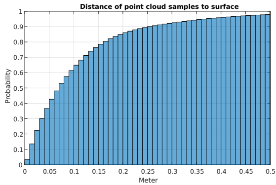
Fig. 11. Histogram of point cloud deviation
