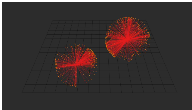
Fig. 2. Extended hedgehogs with unit length splay shots
