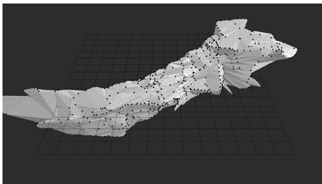
Fig. 5. Voxelized union of turtles
